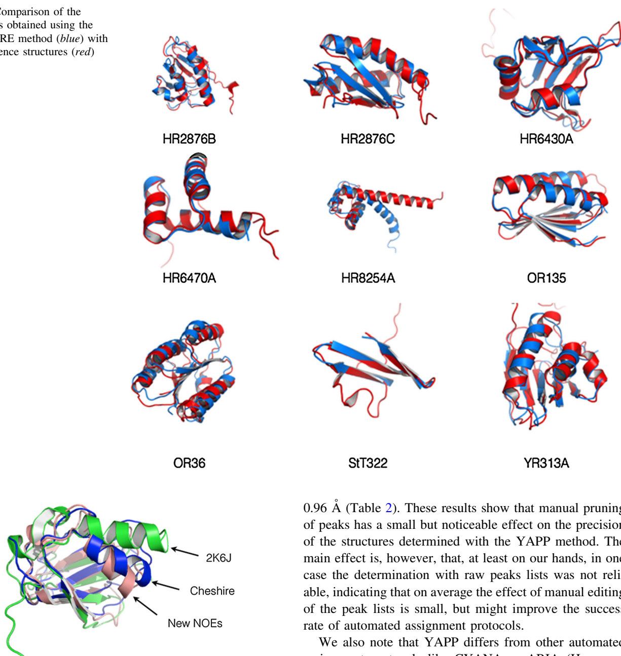
Fig. 3 Comparison of the structures 2K6J, the new NOESY-based structure and the CHESHIRE structure from CASD NMR round 2
