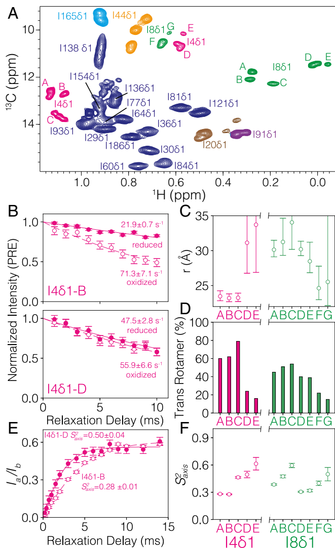
Fig. 2. NMR studies reveal multiple conformers, especially for the N-domain. (A) The Ile region of a ^1\text{H} - ^{13}\text{C} HMQC correlation map of WT SaClpP, 40 °C, 18.8 T, with assignments. Peaks derived from the same residue are colored identically. (B) Representative decay curves for the slowly relaxing component of methyl ^1\text{H} transverse magnetization (circles) along with fits (solid and dashed curves) for a pair of Ile-4 peaks for spin-label oxidized (empty circles) and reduced states (filled circles). Relaxation rates and their uncertainties are displayed for each measurement. (C) Effective distances, r , between the \text{C}^\beta carbon of position 130 (the site of attachment of a TEMPO maleimide spin label) and Ile-4/Ile-8 \delta 1 methyl groups from different conformers, as indicated. (D) Populations of Ile \chi_2 trans rotameric states based on Ile ^{13}\text{C}^{\delta 1} chemical shifts of each of the conformers (56). (E and F) Representative profiles of ratios of peak intensities in triple-quantum-filtered ( I_a ) and single-quantum-based ( I_b ) ^1\text{H} relaxation experiments, I_a/I_b , as a function of relaxation delay (E) along with fits of data to extract the methyl axis order parameter S^2_{\text{axis}} plotted for the Ile-4 and Ile-8 \delta 1 methyl groups as a function of conformer (F).
